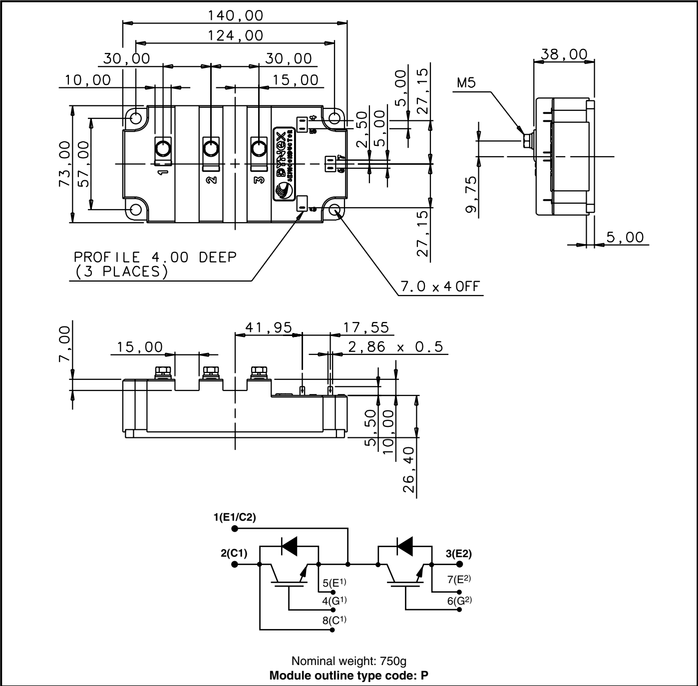
Fig. 11 Package details
