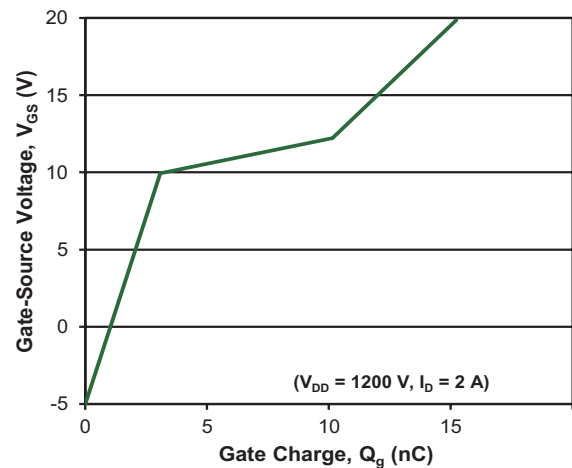
Figure 18: Gate Charge
