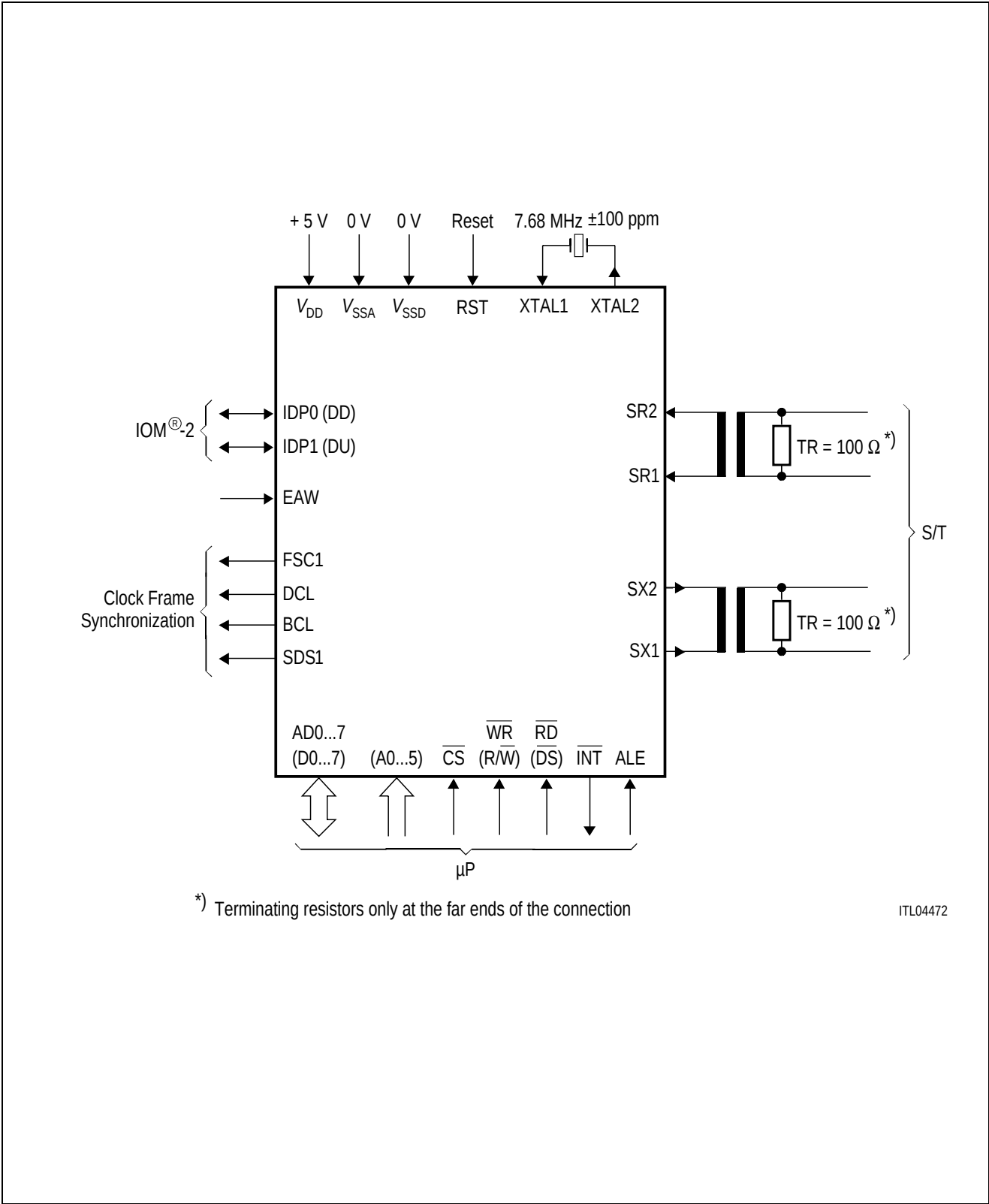
Figure 1 Logic Symbol of the ISAC®-S TE PSB 2186
