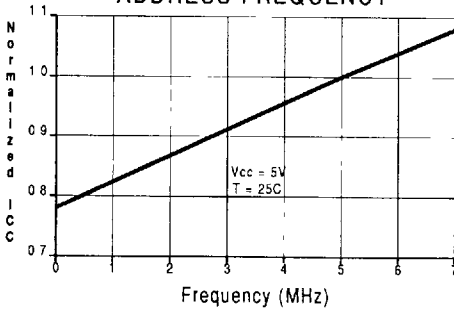
NORMALIZED SUPPLY CURRENT vs. ADDRESS FREQUENCY
