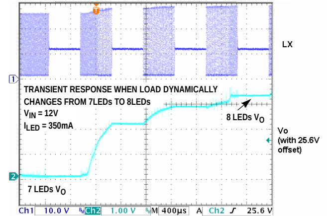
FIGURE 24. TRANSIENT RESPONSE OPERATES FROM 7 TO 8 LEDs
