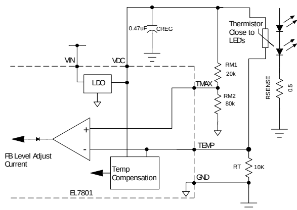
FIGURE 34. OVER-TEMPERATURE CIRCUIT
