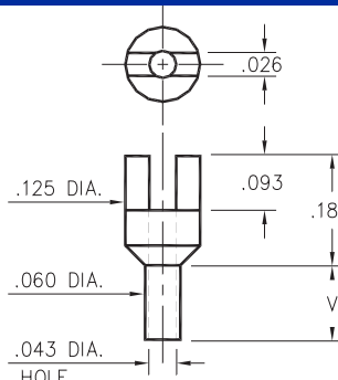
2517-X-01-XX-00-00-07-0 Swage mount in .064 hole
