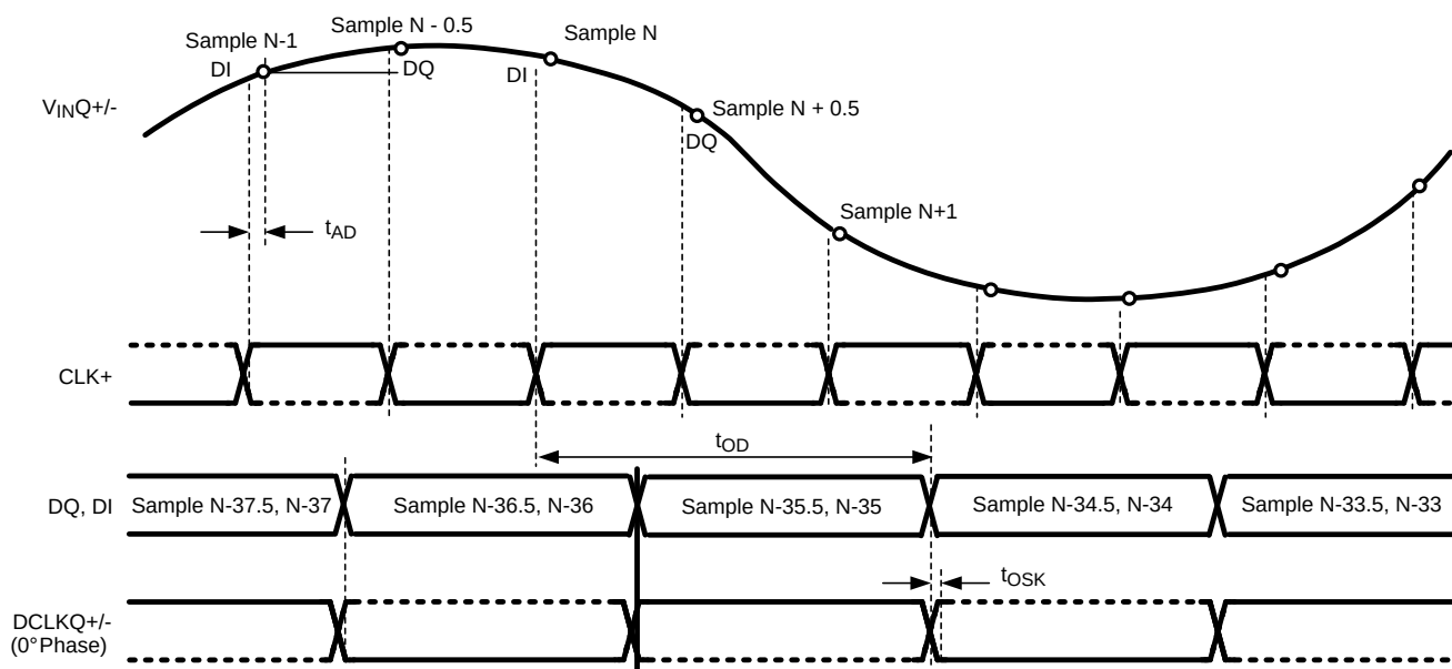
Figure 8. Clocking in Non-Demux Mode DES Mode (See note at Figure 5 )
