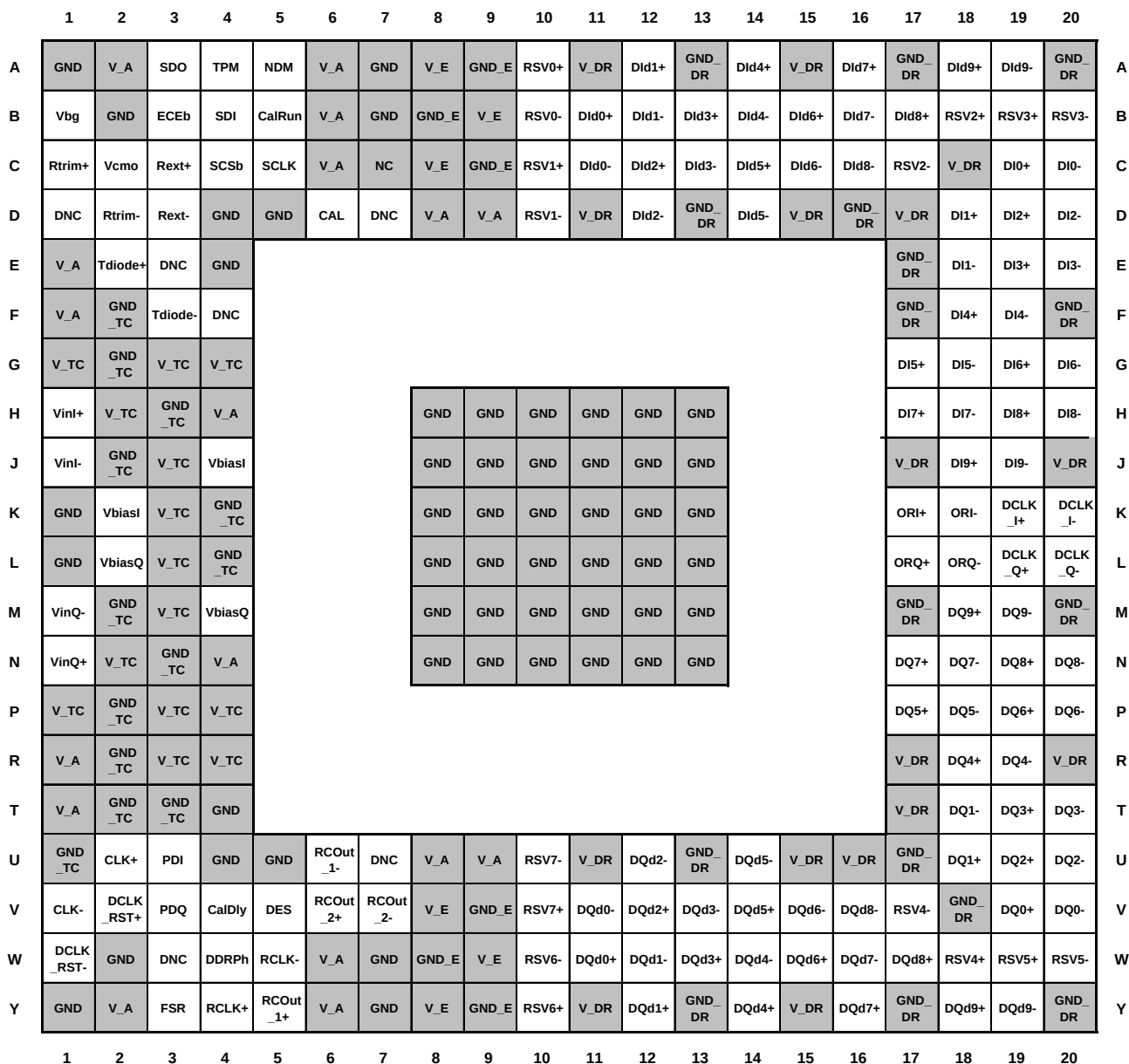
Figure 2. ADC10D1000/1500 Connection Diagram
