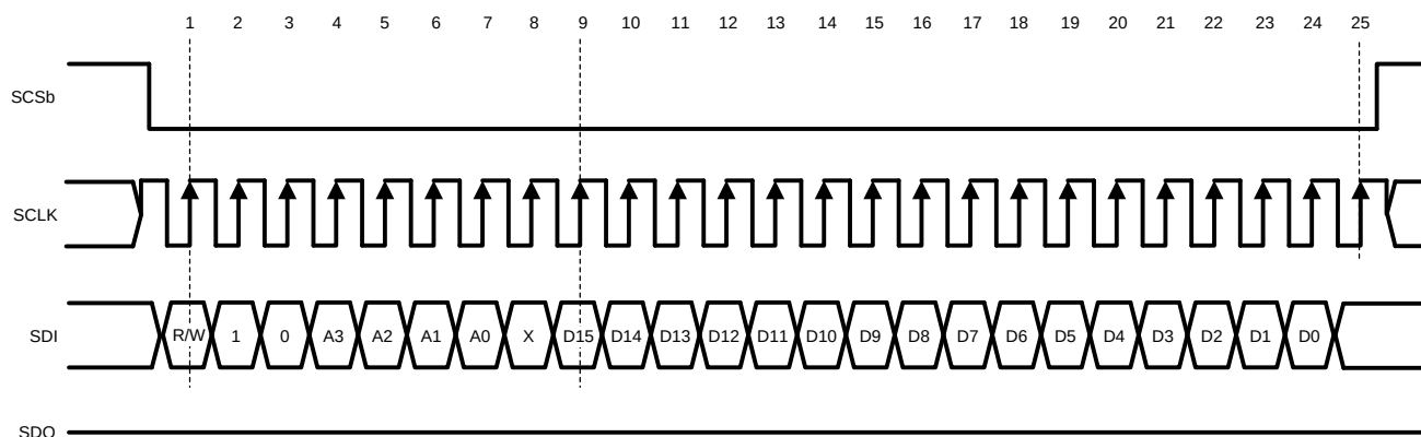
Figure 68. Serial Data Protocol - Write Operation
