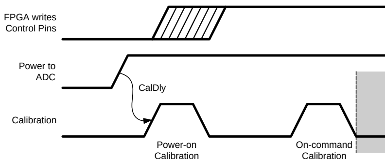
Figure 80. Power-on with Control Pins set by FPGA post Power-on Cal
