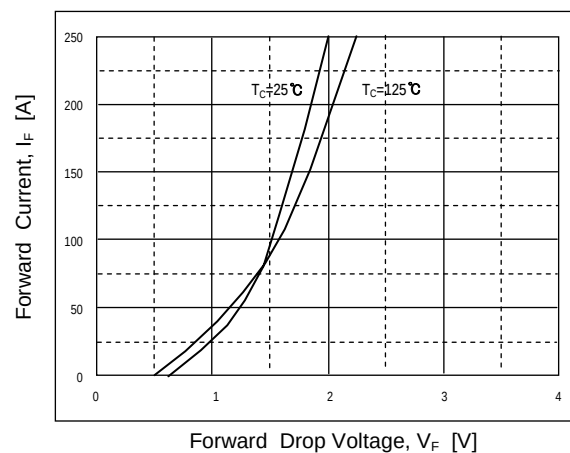
Fig 12. Forward characteristics
