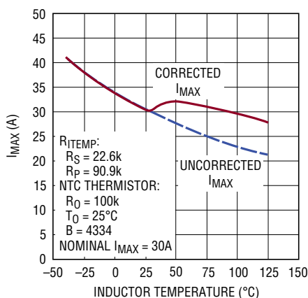
Figure 5. Worst-Case I_{MAX} Versus Inductor Temperature Curve with and without NTC Temperature Compensation
