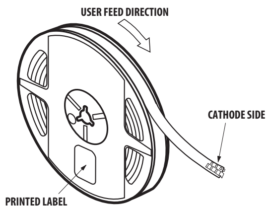
Figure 15. Reeling Orientation
