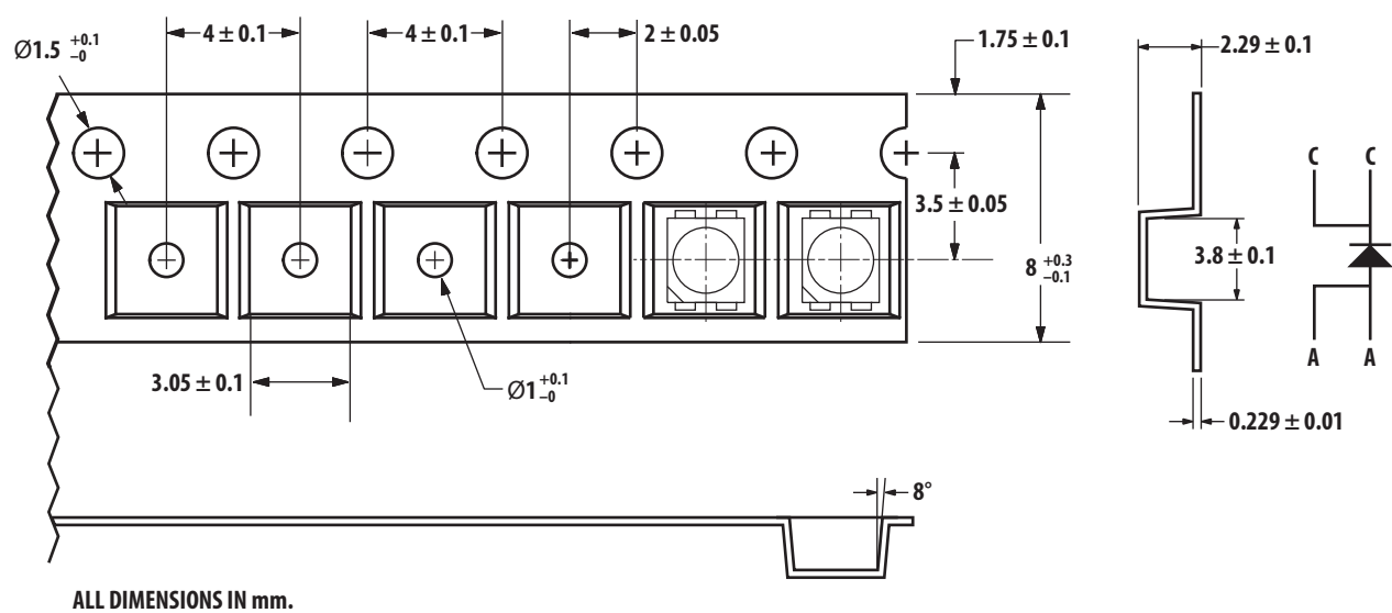
Figure 14. Tape Dimensions
