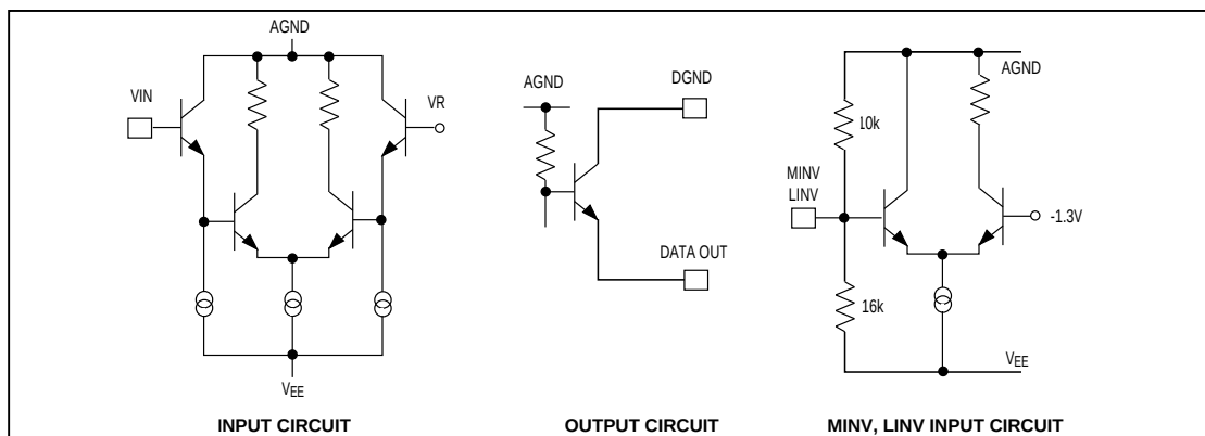
Figure 4. Subcircuit Schematics
