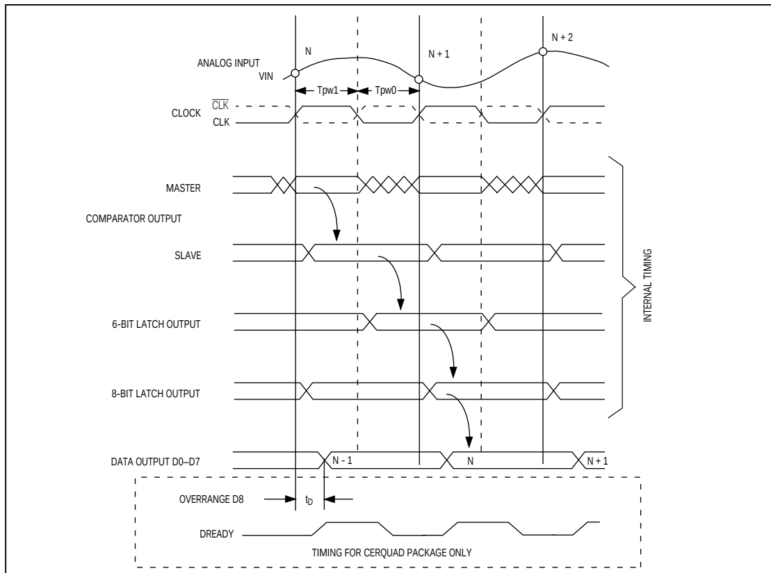
Figure 3. Timing Diagram
