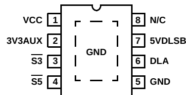
ISL6506 (8 LD EPDIOIC) TOP VIEW
