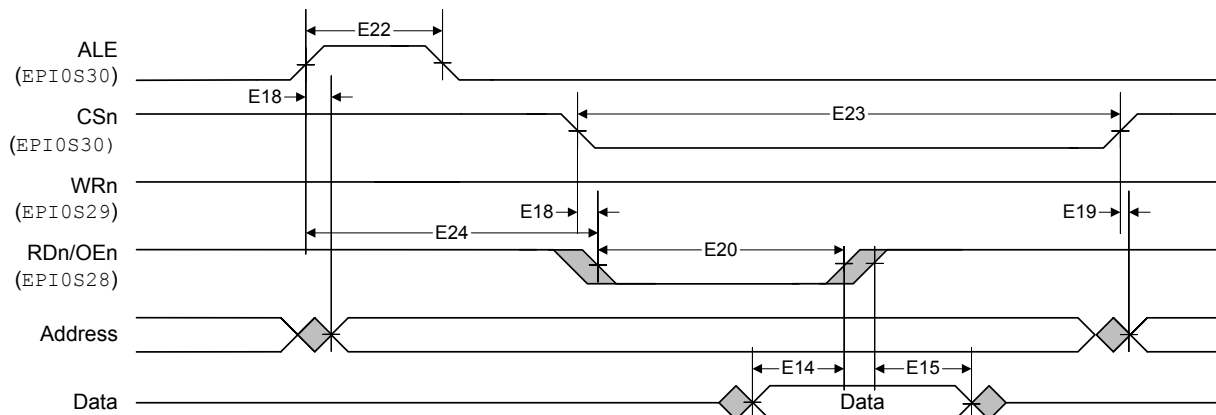
Figure 27-13. Host-Bus 8/16 Mode Read Timing
