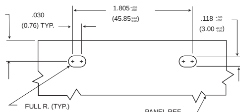
Figure 3 Edgeboard Mounting
