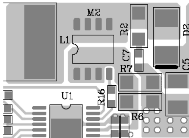
Figure 5—Layout Consideration
