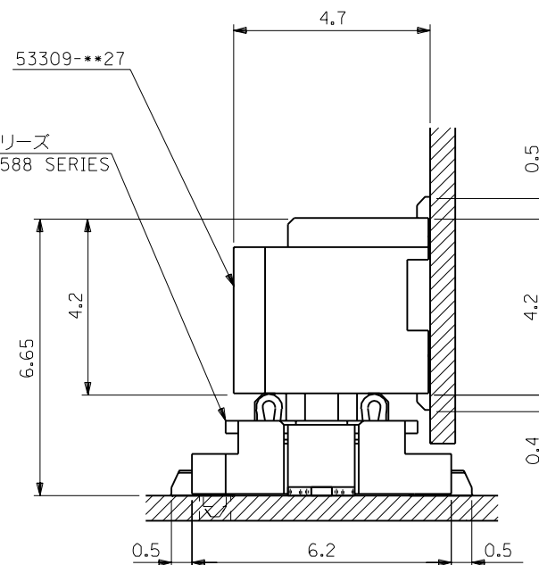
MATED DRAWING(REF.)
