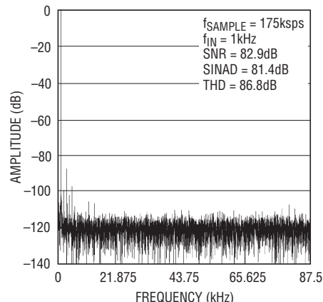
4096 Points FFT Plot ( V_{DD} = 2.7\text{V} , Internal REF)
