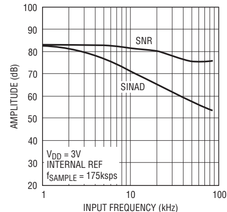
Signal-to-(Noise + Distortion) Ratio vs Input Frequency
