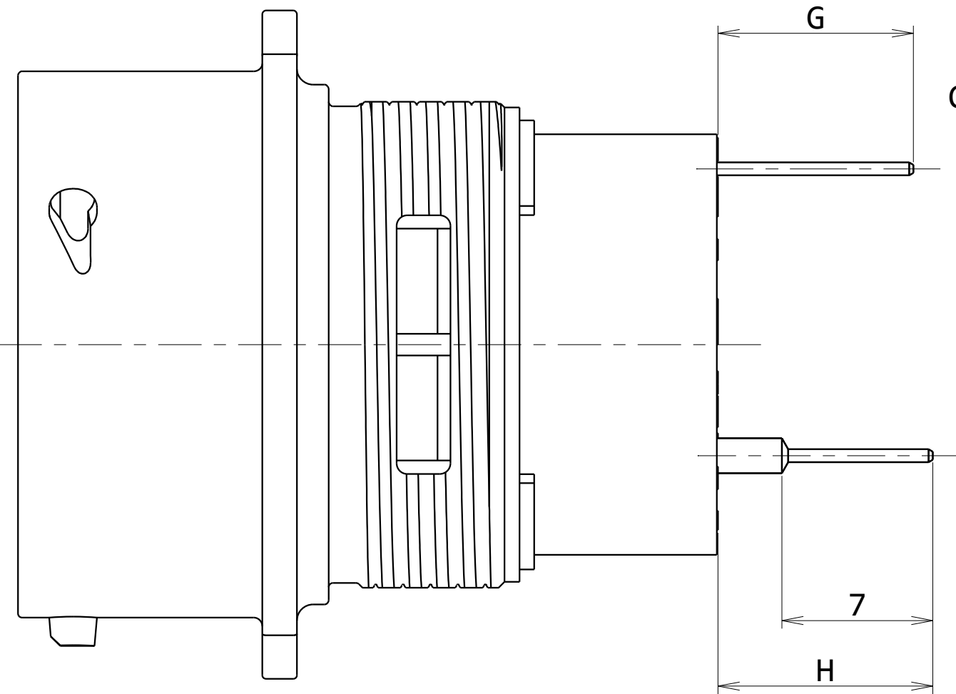
CONTACT TYPE 50-A7
