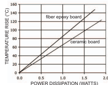
POWER DERATING
