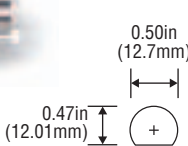
Panel Cut-Out for 4661
