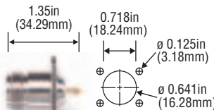
Panel Cut-Out for 2455
