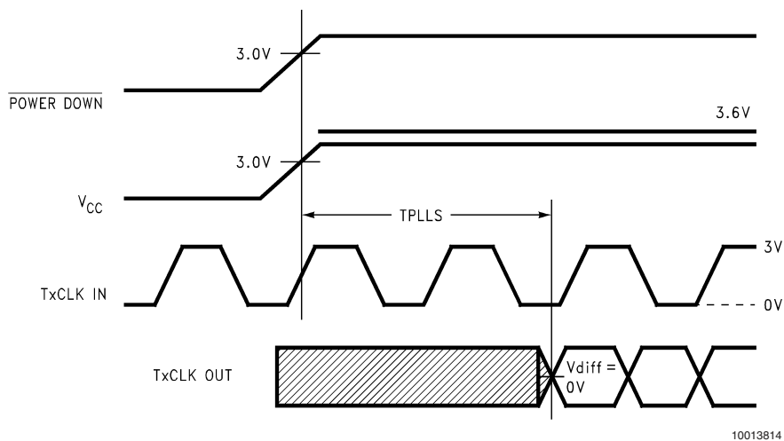
FIGURE 8. DS90C363A/DS90CF363A (Transmitter) Phase Lock Loop Set Time
