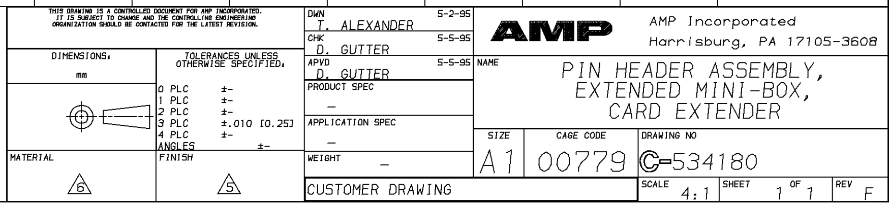
1 & 100 2.900 [73.66] 2.290 [58.17] 2.450 [62.23] 49 2.825 [71.76] 5.650 [143.51] 5.190 [131.83] 5.890 [149.61] 6.050 [153.67] 200 534180-8 1 & 96 2.800 [71.12] 2.190 [55.63] 2.350 [59.69] 47 2.725 [69.22] 5.450 [138.43] 4.990 [126.75] 5.690 [144.53] 5.850 [148.59] 192 534180-7 1 & 90 2.650 [67.31] 2.040 [51.82] 2.200 [55.88] 44 2.575 [65.41] 5.150 [130.81] 4.690 [119.13] 5.390 [136.91] 5.550 [140.97] 180 534180-6 1 & 86 2.550 [64.77] 1.940 [49.28] 2.100 [53.34] 42 2.475 [62.87] 4.950 [125.73] 4.490 [114.05] 5.190 [131.83] 5.350 [135.89] 172 534180-5 1 & 80 2.400 [60.96] 1.790 [45.47] 1.950 [49.53] 39 2.325 [64.46] 4.650 [118.11] 4.190 [106.43] 4.890 [124.21] 5.050 [128.27] 160 534180-4 1 & 76 2.300 [58.42] 1.690 [42.93] 1.850 [46.99] 37 2.225 [56.52] 4.450 [113.03] 3.990 [101.35] 4.690 [119.13] 4.850 [123.19] 152 534180-3 1 & 70 2.150 [54.61] 1.540 [39.12] 1.700 [43.18] 34 2.075 [52.71] 4.150 [105.41] 3.690 [93.73] 4.390 [111.51] 4.550 [115.57] 140 534180-2 1 & 66 2.050 [52.07] 1.440 [36.58] 1.600 [40.64] 32 1.975 [50.17] 3.950 [100.33] 3.490 [88.65] 4.190 [106.43] 4.350 [110.49] 132 534180-1 CAVITY IDENT. I H G F E D C B A POSN. PART NO.
