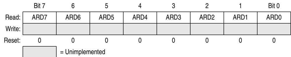
Figure 13-19. ESCI Arbiter Data Register (SCIADAT)
