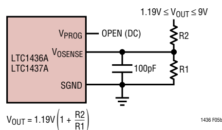
Figure 5b. LTC1436A/LTC1437A Adjustable Applications
