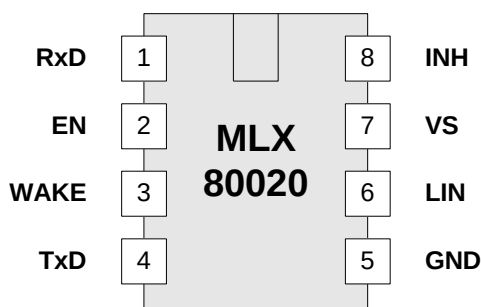
Figure 2: Pin description SOIC8 package
