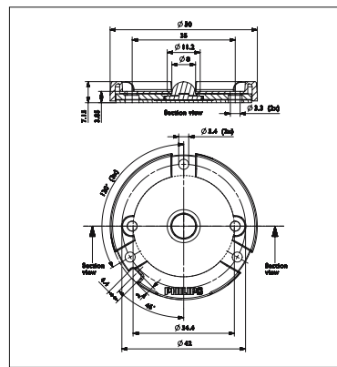
Fortimo LED Spotlight Module Tight Beam
