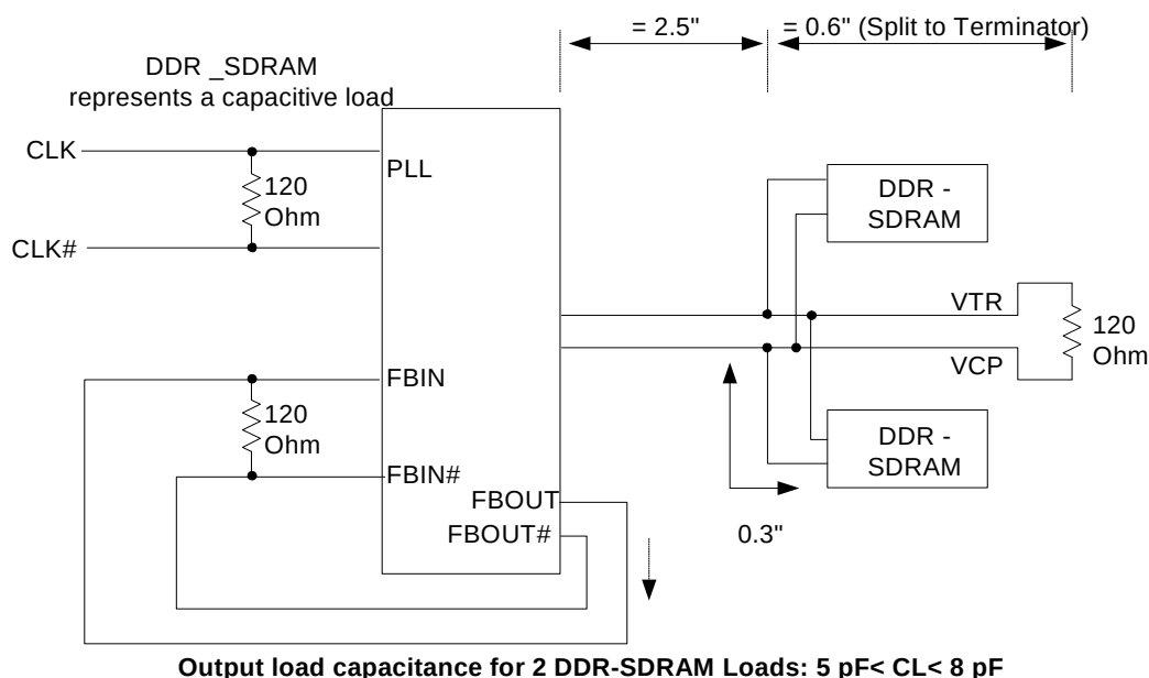
Figure 4. Clock Structure # 1
