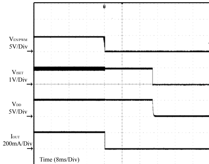
Figure 26 EN/PWM Disable
