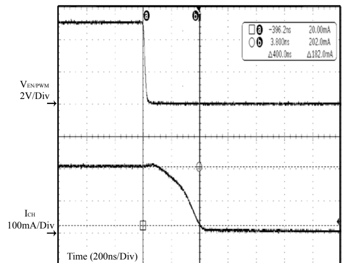
Figure 25 EN/PWM Falling
