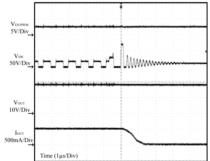
Figure 21 Open Schottky Diode During Normal Operation
