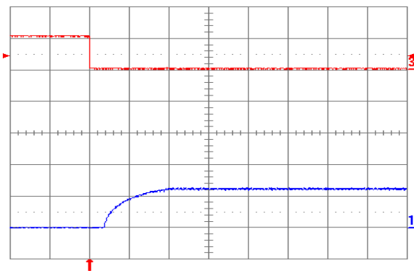
Figure 1.2V.16. Turn-on transient at full rated load current (resistive) plus 10,000 \mu\text{F} at V_{in} = 48\text{ V} , triggered via ON/OFF pin. Top trace: ON/OFF signal (5 V/div.). Bottom trace: output voltage (1 V/div.). Time scale: 2 ms/div.
