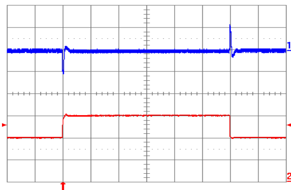
Figure 1.2V.18. Output voltage response to load current step-change (20 A – 30 A – 20 A) at V_{in} = 48\text{ V} . Top trace: output voltage (100 mV/div.). Bottom trace: load current (10 A/div.). Current slew rate: 5 A/ \mu\text{s} . C_o = 470\text{ }\mu\text{F POS} + 1\text{ }\mu\text{F ceramic} . Time scale: 0.2 ms/div.
