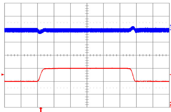
Figure 1.2V.17. Output voltage response to load current step-change (20 A – 30 A – 20 A) at V_{in} = 48\text{ V} . Top trace: output voltage (100 mV/div.). Bottom trace: load current (10 A/div.). Current slew rate: 0.1 A/ \mu\text{s} . C_o = 1\text{ }\mu\text{F} ceramic. Time scale: 0.2 ms/div.
