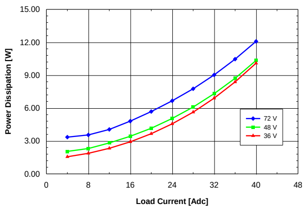
Figure 1.2V.13. Power dissipation vs. load current and input voltage for QME48T40012 converter mounted horizontally with air flowing from pin 1 to pin 3 at a rate of 300 LFM (1.5 m/s) and T_a = 25\text{ }^{\circ}\text{C} .
