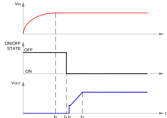
Figure 6. Startup scenario #2.
