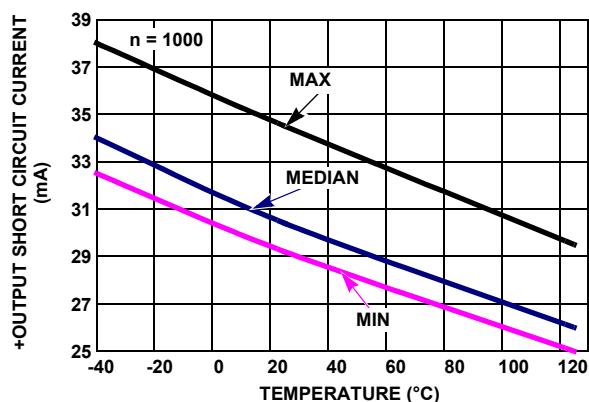
FIGURE 35. +OUTPUT SHORT CIRCUIT CURRENT vs TEMPERATURE V_{IN} = +2.5V , R_L = 10 , V_+ = 5V , V_- = \pm 2.5V
