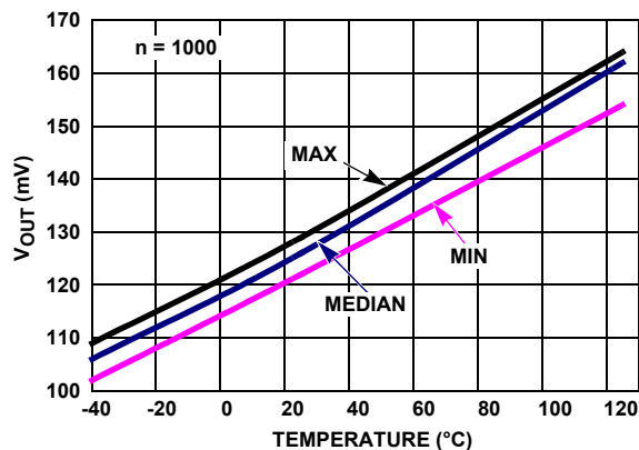
FIGURE 33. V_{OUT} LOW vs TEMPERATURE, V_+ = 5V , V_- = \pm 2.5V , R_L = 1k
