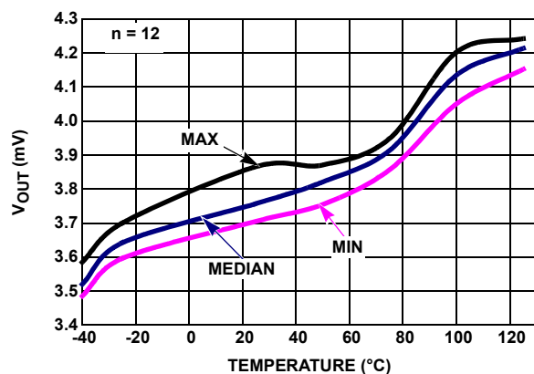
FIGURE 34. V_{OUT} LOW vs TEMPERATURE, V_+ = 5V , V_- = \pm 2.5V , R_L = 100k
