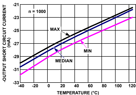
FIGURE 36. -OUTPUT SHORT CIRCUIT CURRENT vs TEMPERATURE V_{IN} = -2.5V , R_L = 10 , V_+ = 5V , V_- = \pm 2.5V
