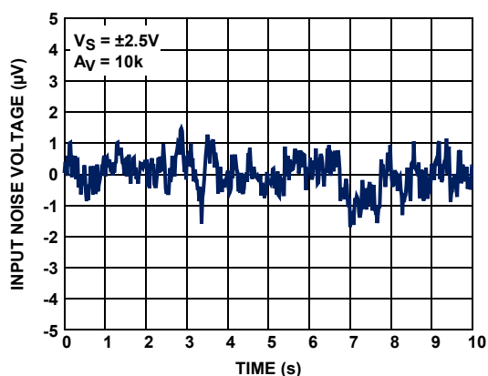
FIGURE 12. 0.1Hz TO 10Hz INPUT VOLTAGE NOISE
