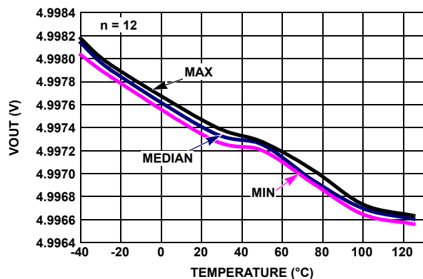
FIGURE 32. V_{OUT} HIGH vs TEMPERATURE, V_+ = 5V , V_- = \pm 2.5V , R_L = 100k
