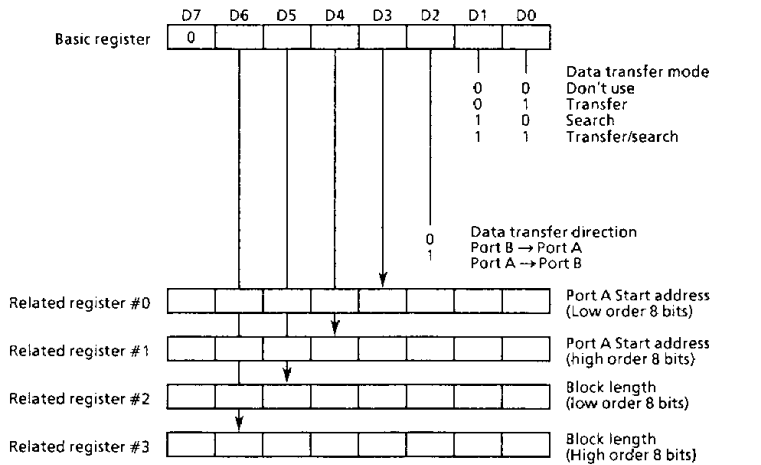
Figure 3.35 Write Register WR0
