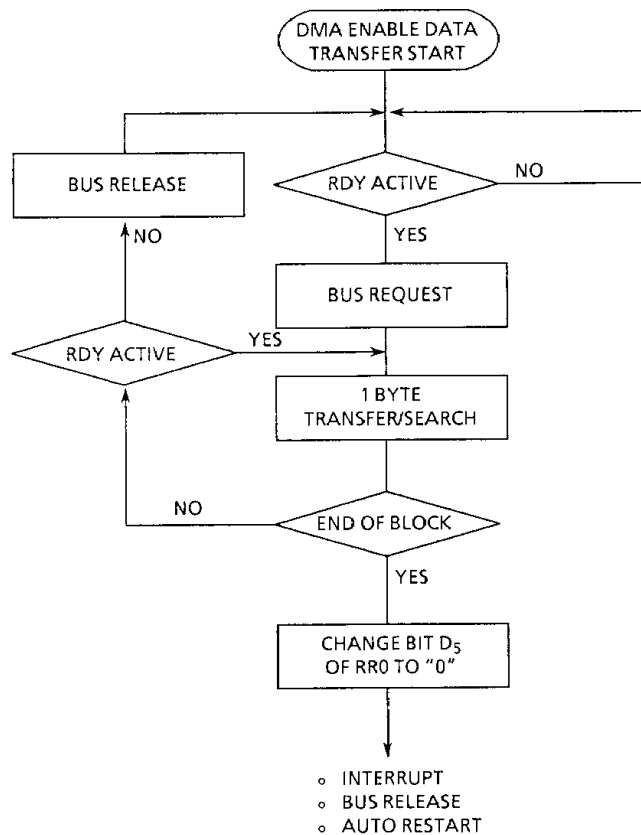
Figure 3.9 Burst Mode
