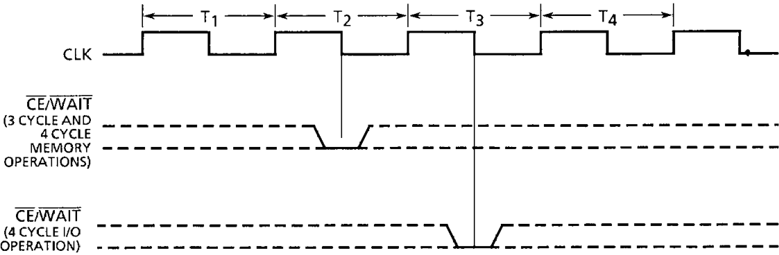
Figure 3.31 WAIT Sample in Variable Timing
