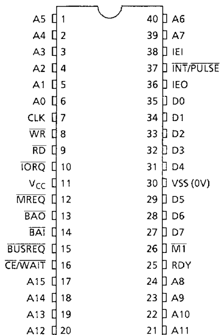
Figure 2.1 DIP, SOP Pin Assignments
