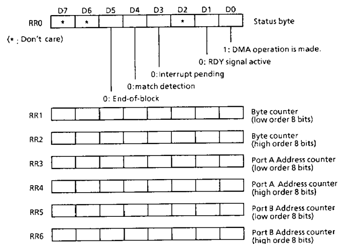
Figure 3.42 Read Register
