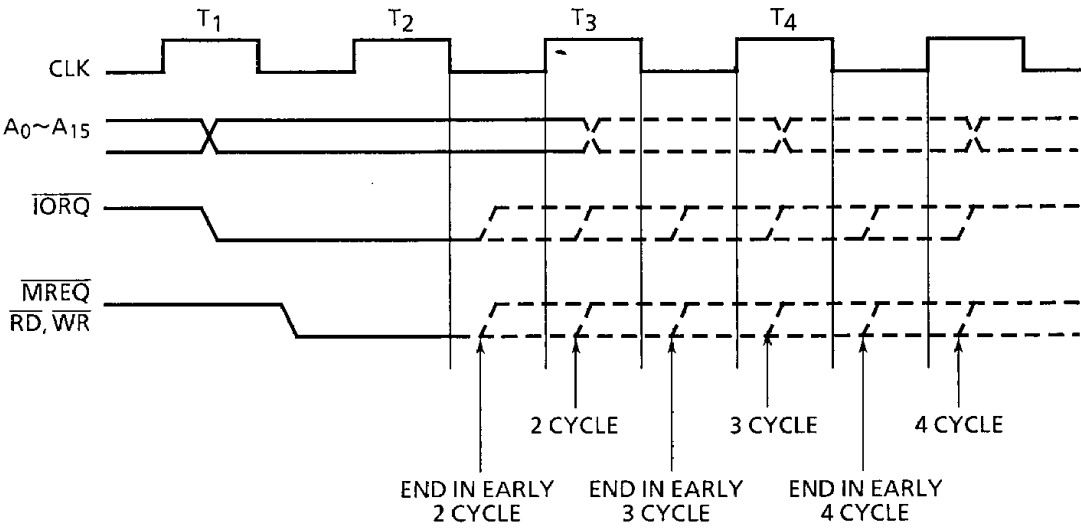
Figure 3.30 Variable Cycle
