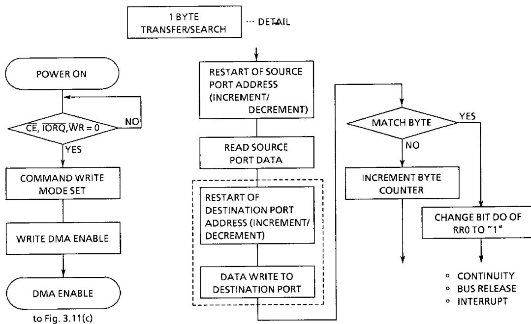
Figure 3.11 (b) Status Change Flowchart
