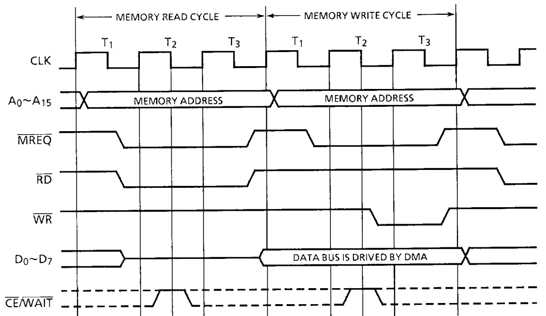
Figure 3.16 Transfer Timing of Memory to Memory
