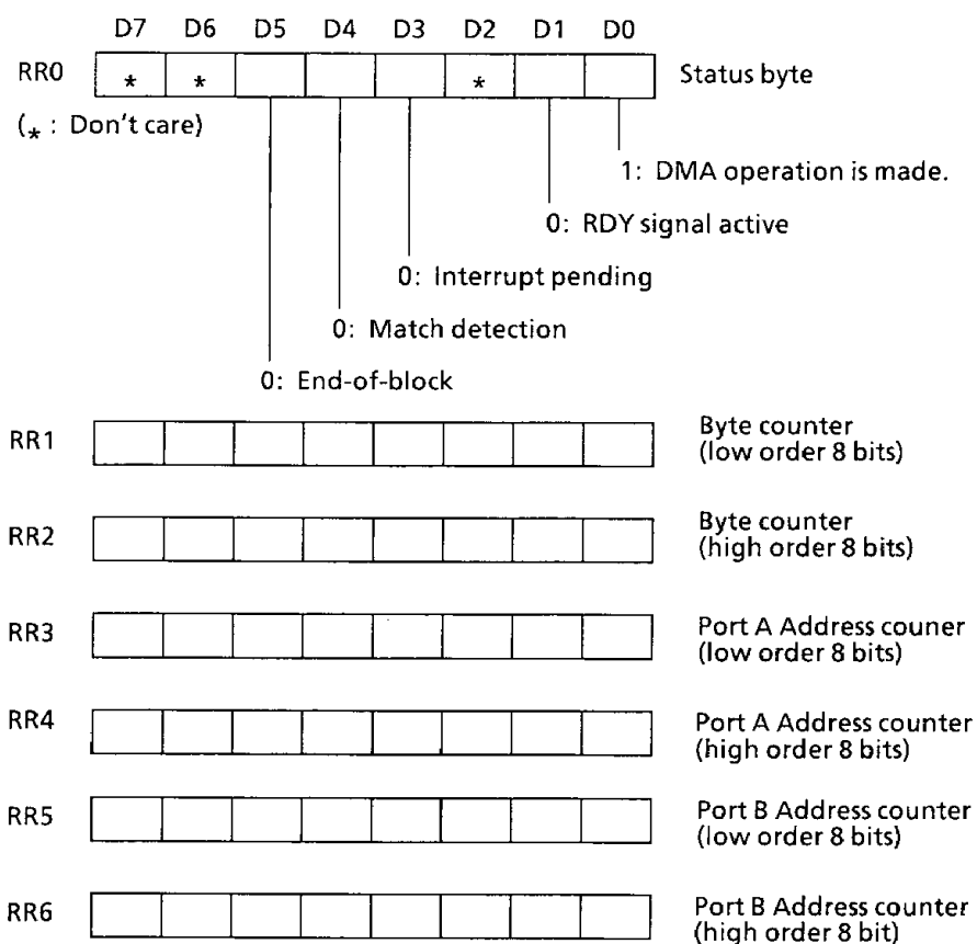
Figure 3.42 Read Register
