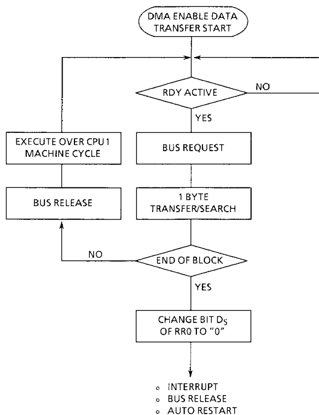
Figure 3.8 Byte Mode
