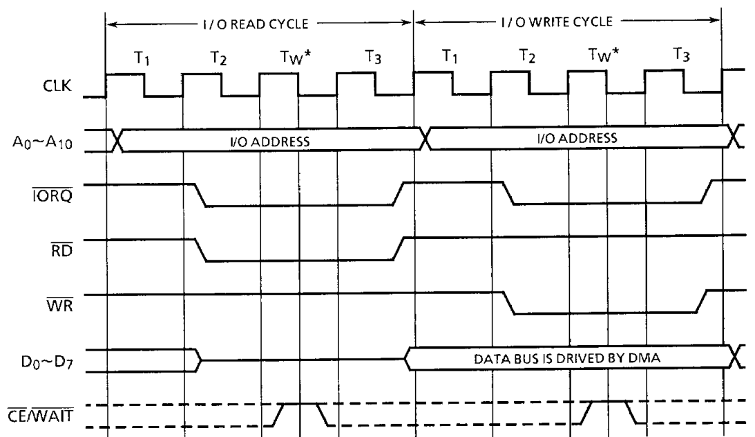
Figure 3.17 Transfer Timing of I/O to I/O
