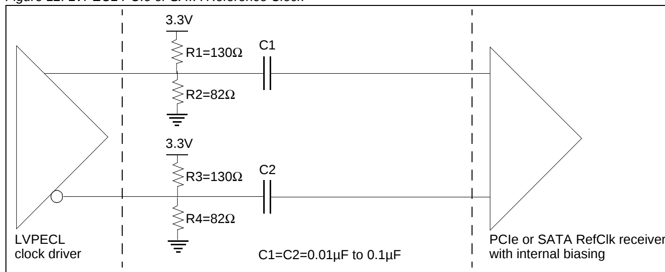
Figure 12. LVPECL PCIe or SATA Reference Clock
