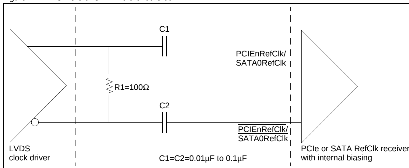
Figure 11. LVDS PCIe or SATA Reference Clock
