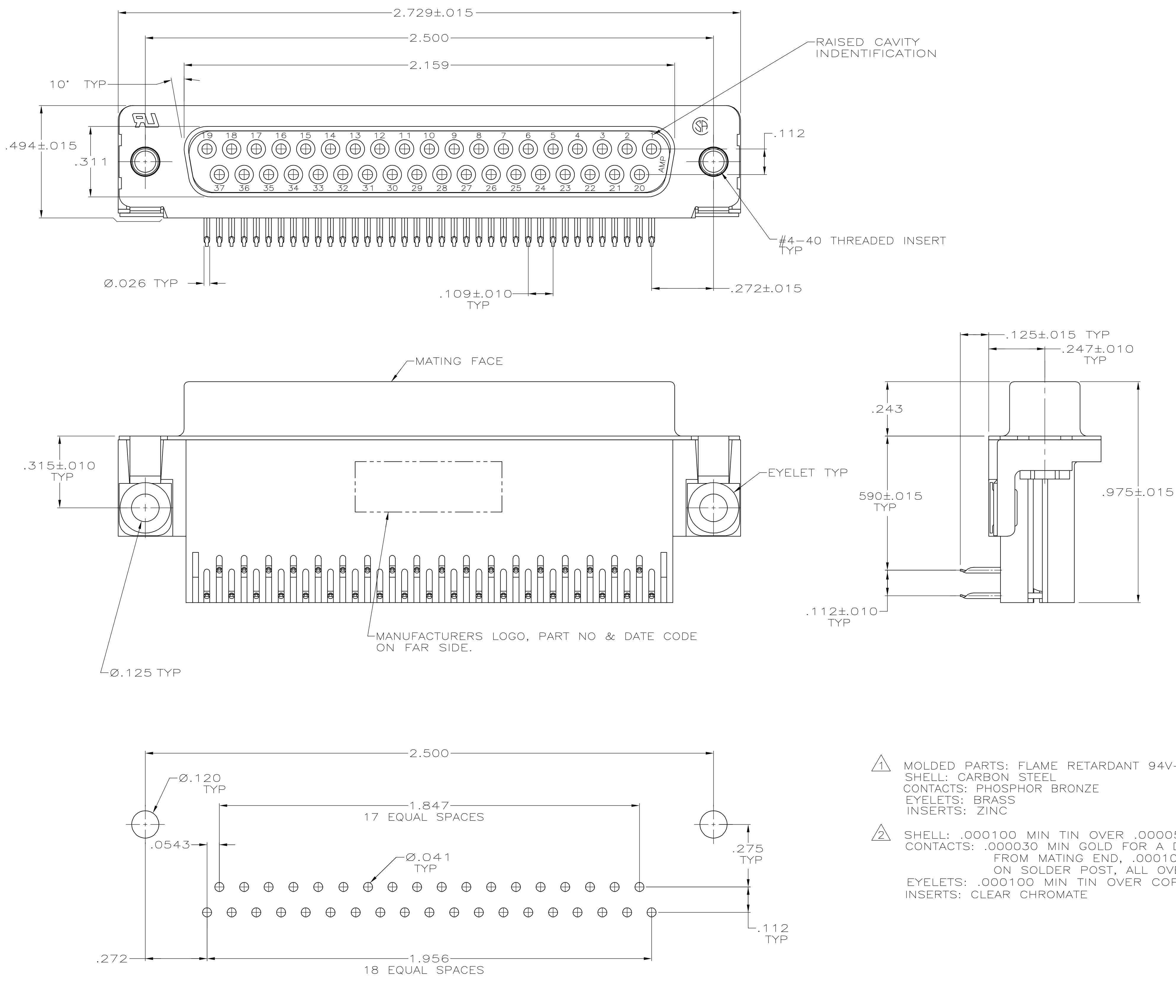
RECOMMENDED P.C. BOARD MOUNTING DIMENSIONS
