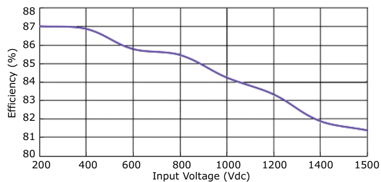
AE40-UW-S24 Efficiency Curve Efficiency vs. Input Voltage
