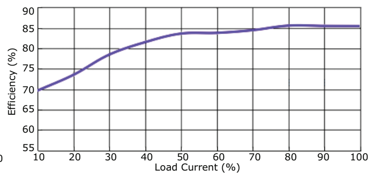
AE40-UW-S24 Efficiency Curve Efficiency vs. Load Current
