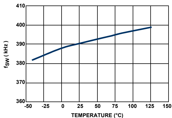
FIGURE 15. SWITCHING FREQUENCY vs TEMPERATURE
