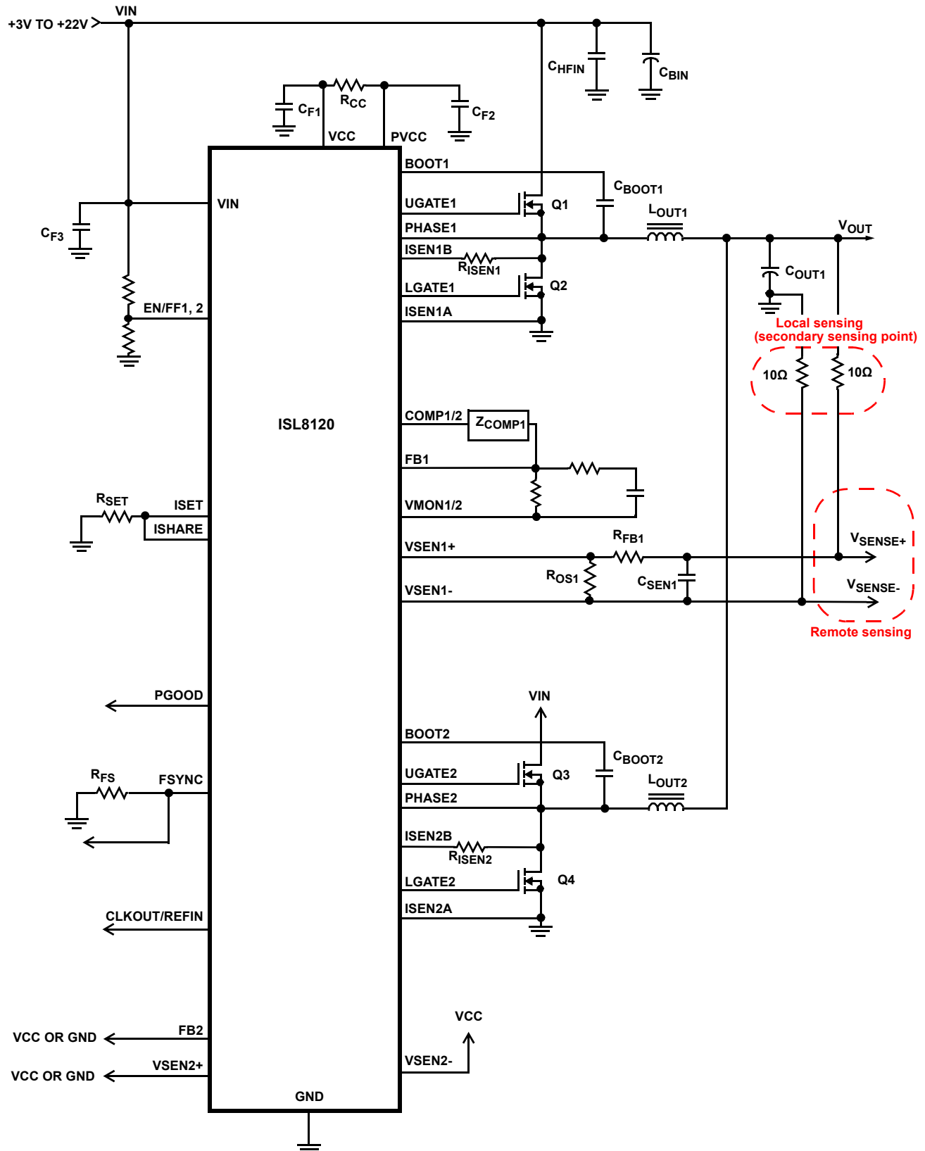
FIGURE 4. 2-PHASE OPERATION WITH r_{DS(ON)} SENSING
