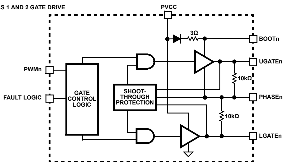
FIGURE 1. INTEGRATED DRIVER BLOCK DIAGRAM
