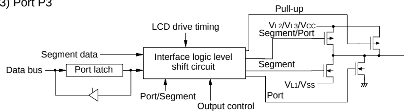
(3) Port P3
