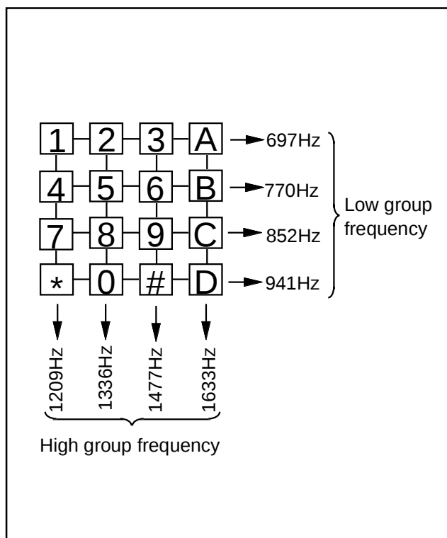
Fig. 41 Key matrix of telephone and rating frequency
