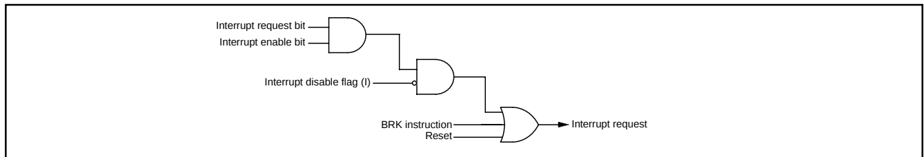
Fig. 17 Interrupt control
