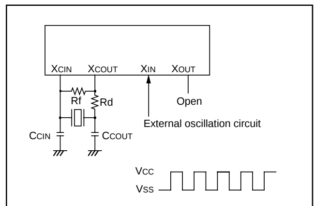
Fig. 56 External clock input circuit
