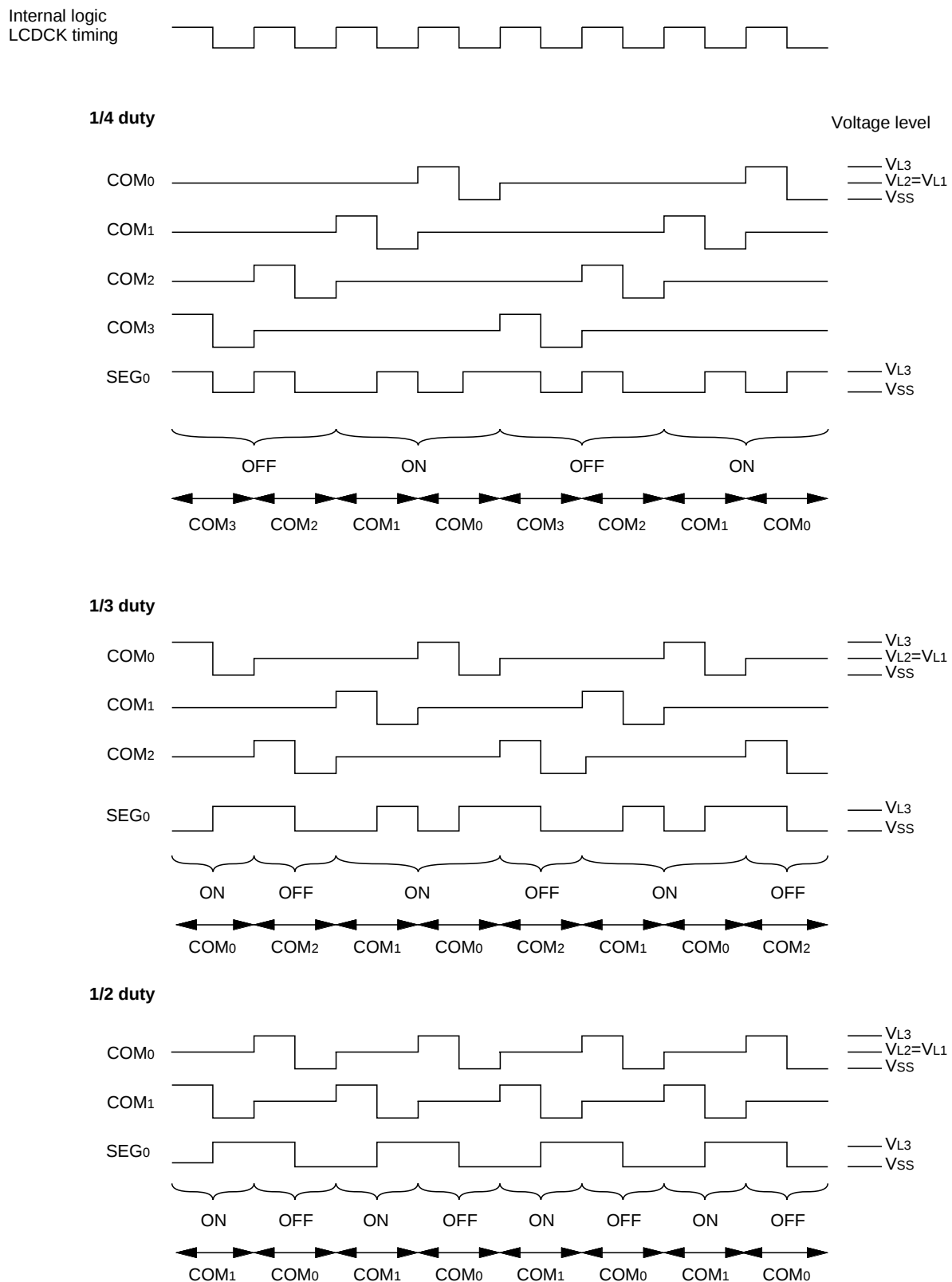
Fig. 46 LCD drive waveform (1/2 bias)
