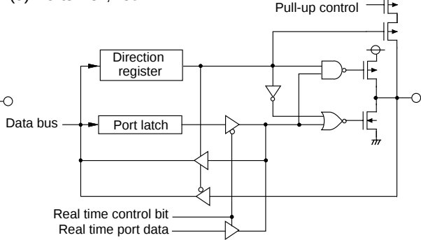
(9) Ports P52,P53
