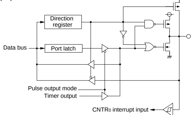
(11) Port P54
