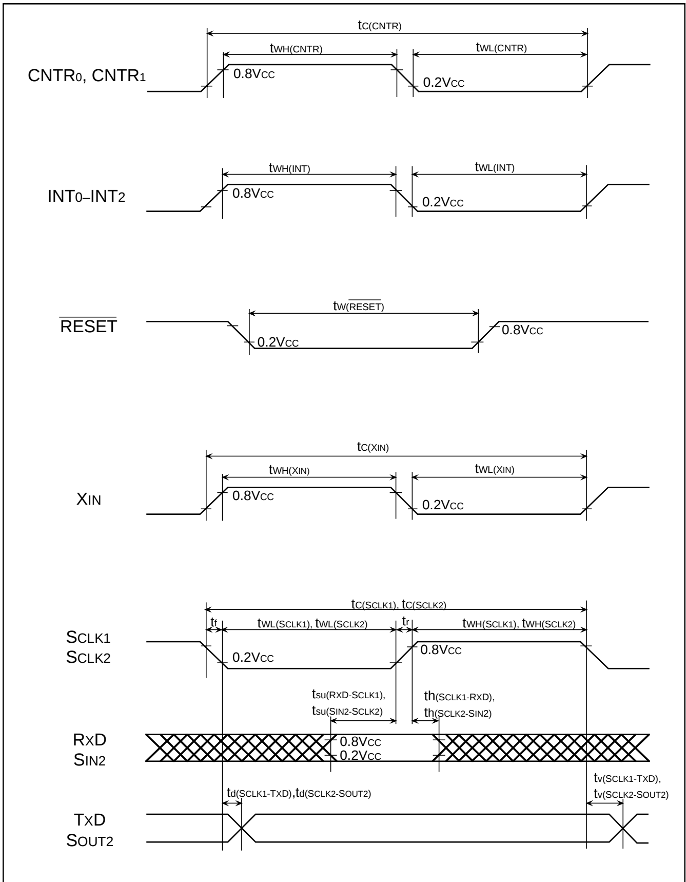
Fig. 61 Timing diagram
