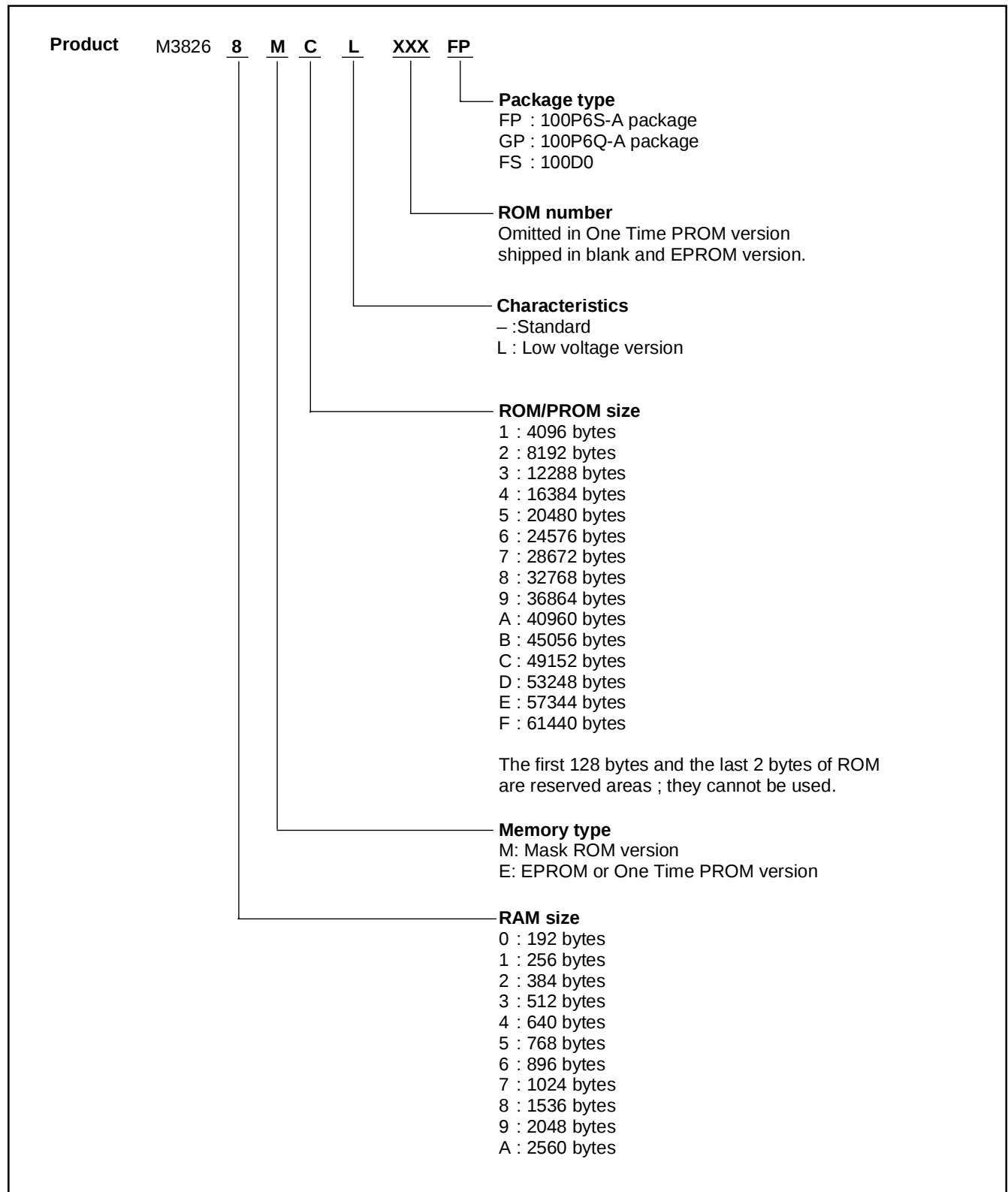
Fig. 4 Part numbering
