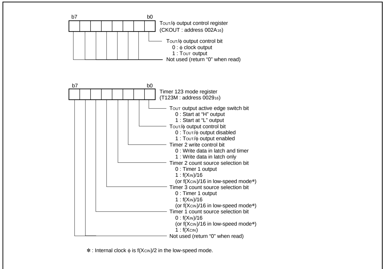
Fig. 51 Structure of TOUT/φ output-related register
