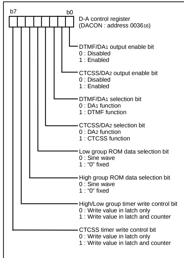
Fig. 38 Structure of D-A control register
