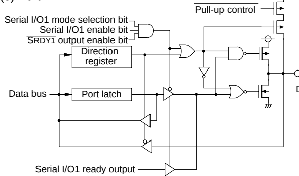
(8) Port P47
