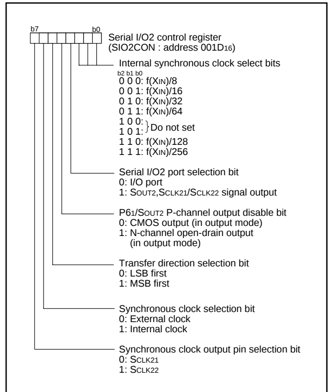
Fig. 29 Structure of serial I/O2 control register
