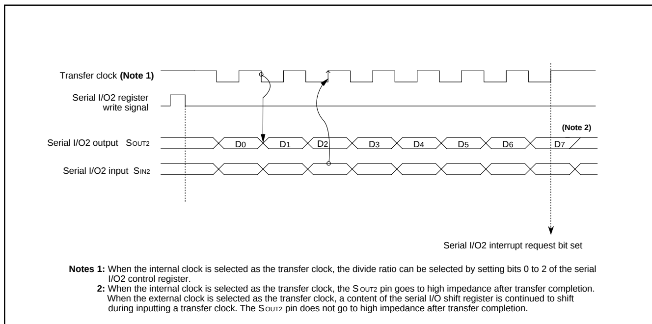
Fig. 31 Timing of serial I/O2 function
