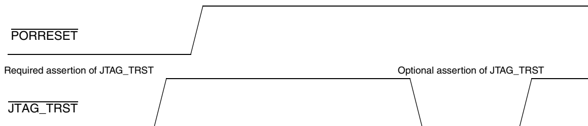
Figure 53. PORRESET vs. JTAG_TRST
