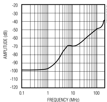
MAX4117-MAX4120 CROSSTALK vs. FREQUENCY
