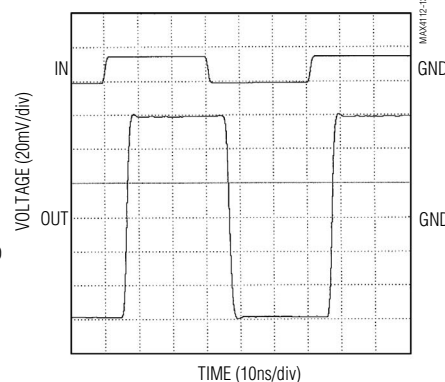
MAX4113/MAX4118/MAX4120 LARGE-SIGNAL PULSE RESPONSE ( A_{vCL} = +20 )
