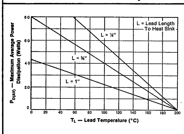
FIGURE 1—Power or Current Derating
