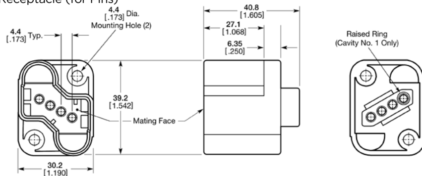
Receptacle (for Pins)
