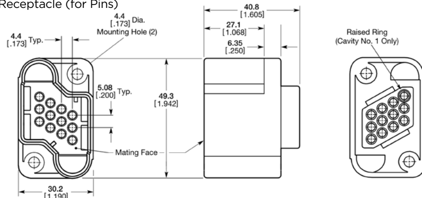
Receptacle (for Pins)
