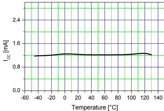
Figure 9. Operating Supply Current vs. Temp.
