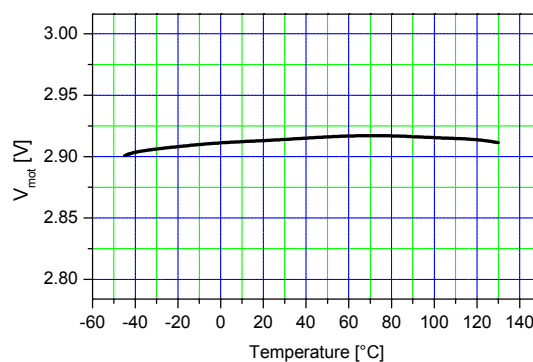
Figure 19. Maximum On-Time Voltage vs. Temp.
