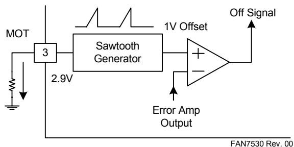
Figure 35. Sawtooth Generator Block
