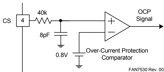
Figure 36. Over-Current Protection Block
