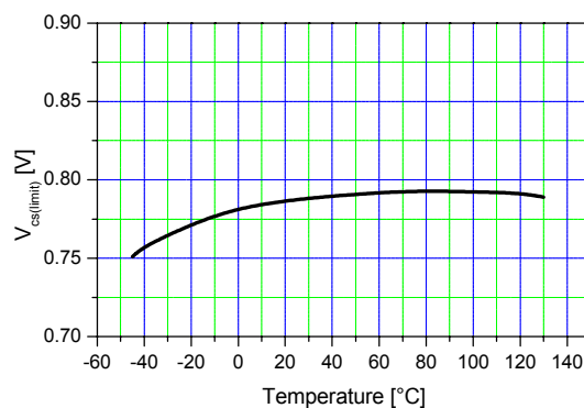
Figure 21. Current Sense Input Threshold Voltage vs. Temp.
