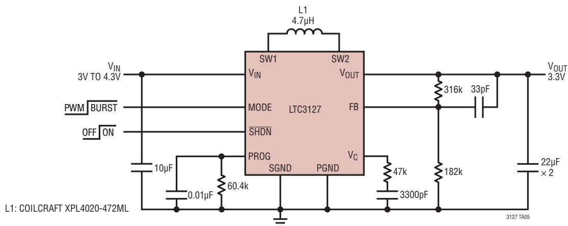
General Purpose Forced Continuous Conduction Application with 500μs Start-Up
