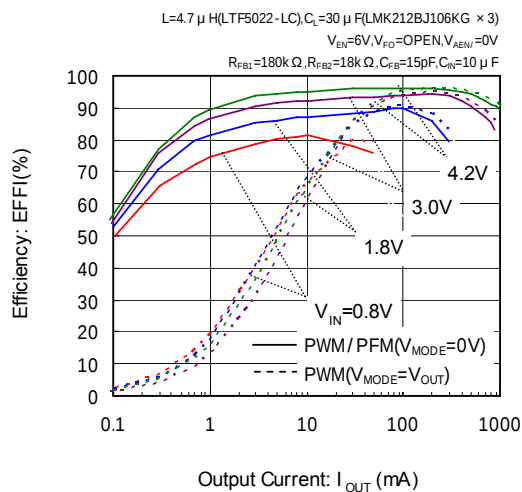
XC9128 ( V_{OUT}=5.0V )
