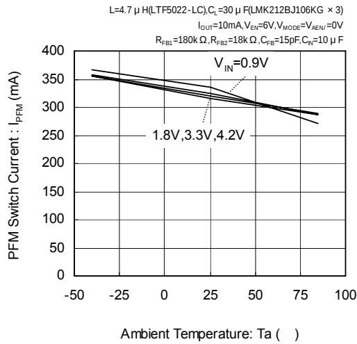
XC9128 ( V_{OUT}=1.8V )
