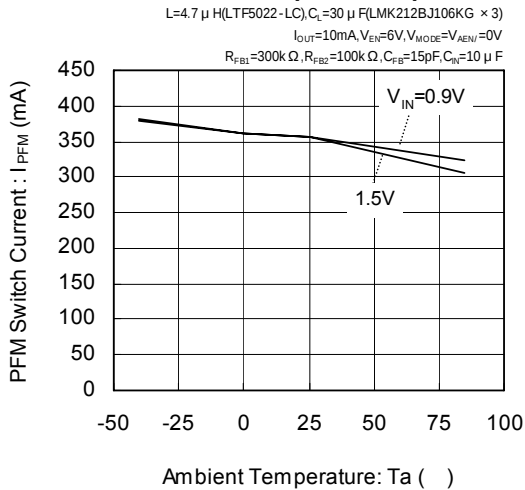
XC9128 ( V_{OUT}=1.8V )
