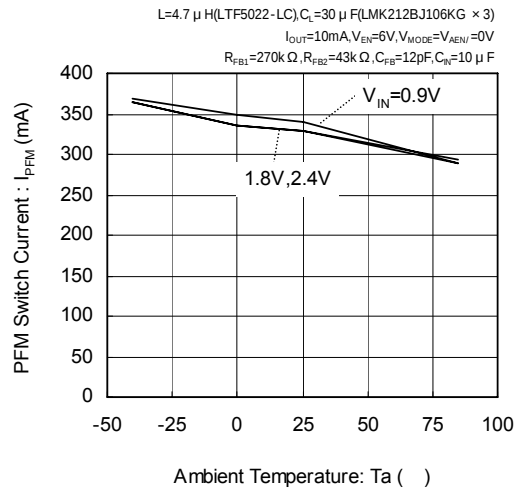
XC9128 ( V_{OUT}=3.3V )
