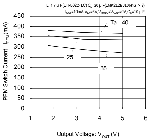
XC9128 ( V_{IN}=0.9V )
