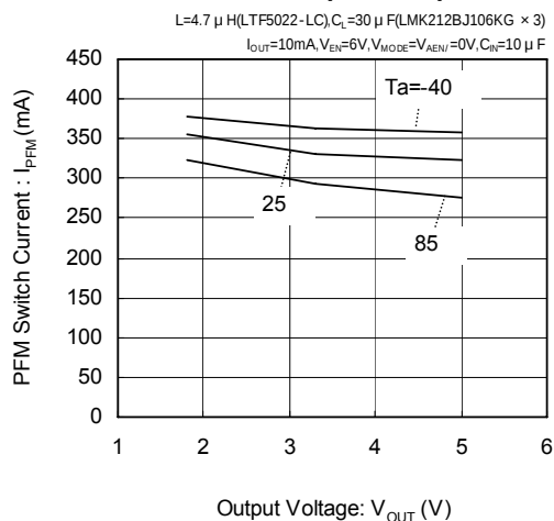
XC9128 ( V_{IN}=1.5V )
