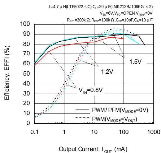
XC9128 ( V_{OUT}=1.8V )
