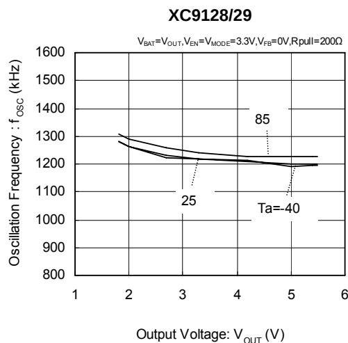
(13) Oscillation Frequency vs. Output Voltage
