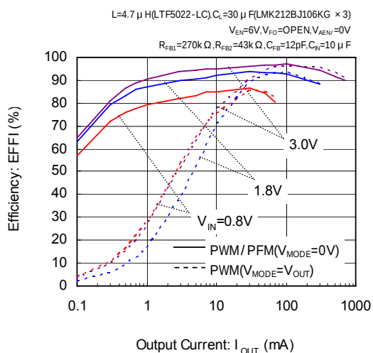
XC9128 ( V_{OUT}=1.8V )
