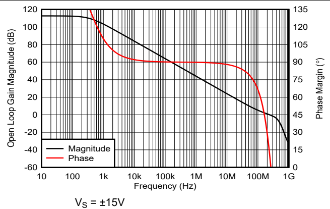
Figure 5-12. Open Loop Frequency Response
