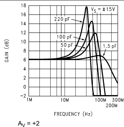
Figure 5-75. Closed-Loop Frequency Response vs Capacitive Load
