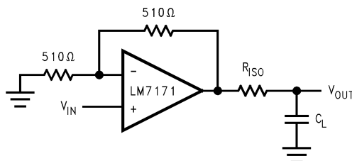
Figure 6-9. Isolation Resistor Used to Drive Capacitive Load
