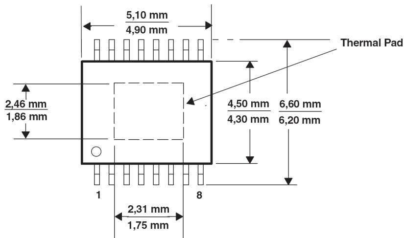
Figure 13. PowerPAD Dimensions
