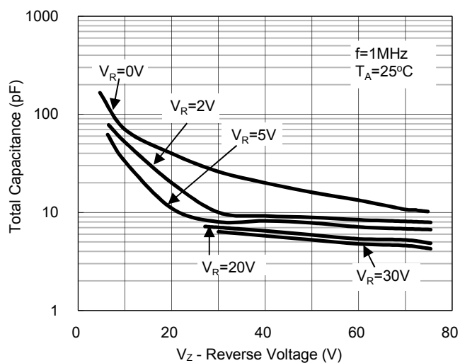
Fig. 2 Total Capacitance
