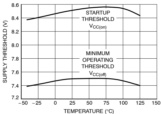
Figure 18. Supply Voltage Thresholds versus Temperature
