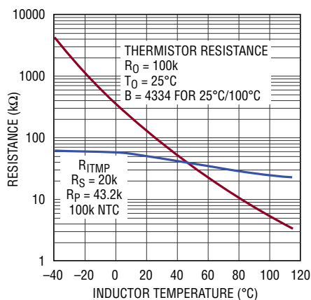
Figure 6. Resistance Versus Temperature for the ITEMP Pin Network and the 100k NTC
