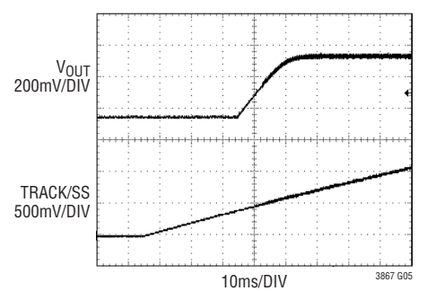
Pre-Bias Start-Up
