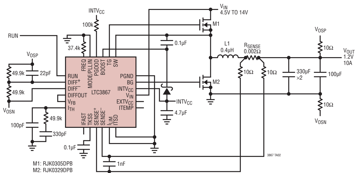
1.2V, 10A Output with R_{\text{SENSE}}
