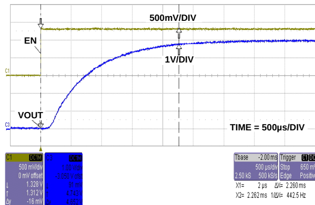
FIGURE 8. START-UP WAVEFORM
