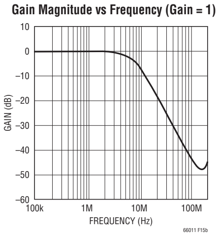
Figure 15. Modified Filter Configuration Using a Resistor Between Summing Nodes ( f_{-3dB} = 7.5\text{MHz} )
